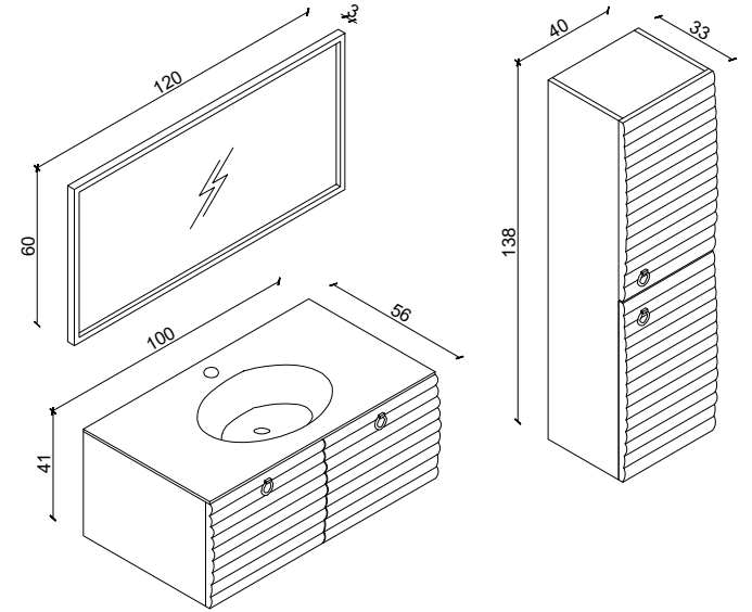
- FLORIDA 100 Lavabo: Camaks (Cam Lavabo 12 mm 100 X 56 cm Siyah)
