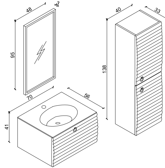
- FLORIDA 70 Lavabo: Camaks (Cam Lavabo 12 mm 70 X 56 cm Siyah)
